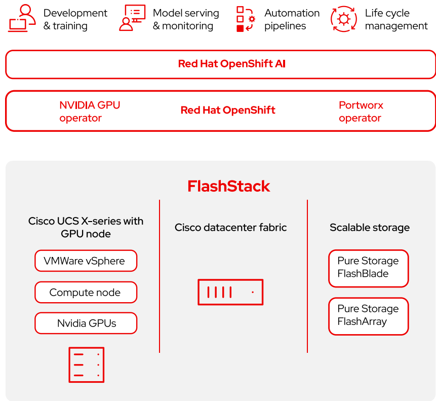
Figure 2. A high-level architecture of the FlashStack AI MLOps solution using Red Hat OpenShift AI.
